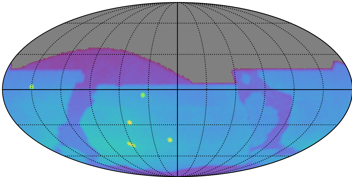
ddf_acor_sf10_lsf30_lsr10_v3.4_10yrs : Brown Dwarf, L4
