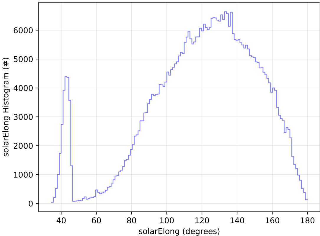
ddf_acor_sf10_ls30_lsr10_v3.4_10yrs WFD z band: solarElong Histogram
