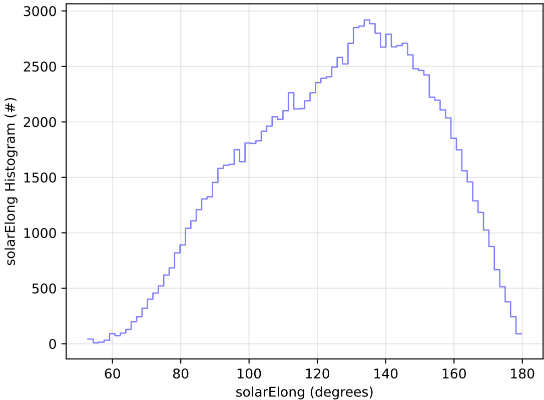
ddf_acor_sf10_lsf30_lsr10_v3.4_10yrs WFD u band: solarElong Histogram
