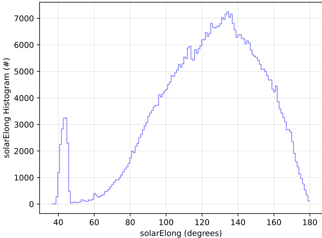
ddf_acor_sf10_ls30_lsr10_v3.4_10yrs WFD r band: solarElong Histogram
