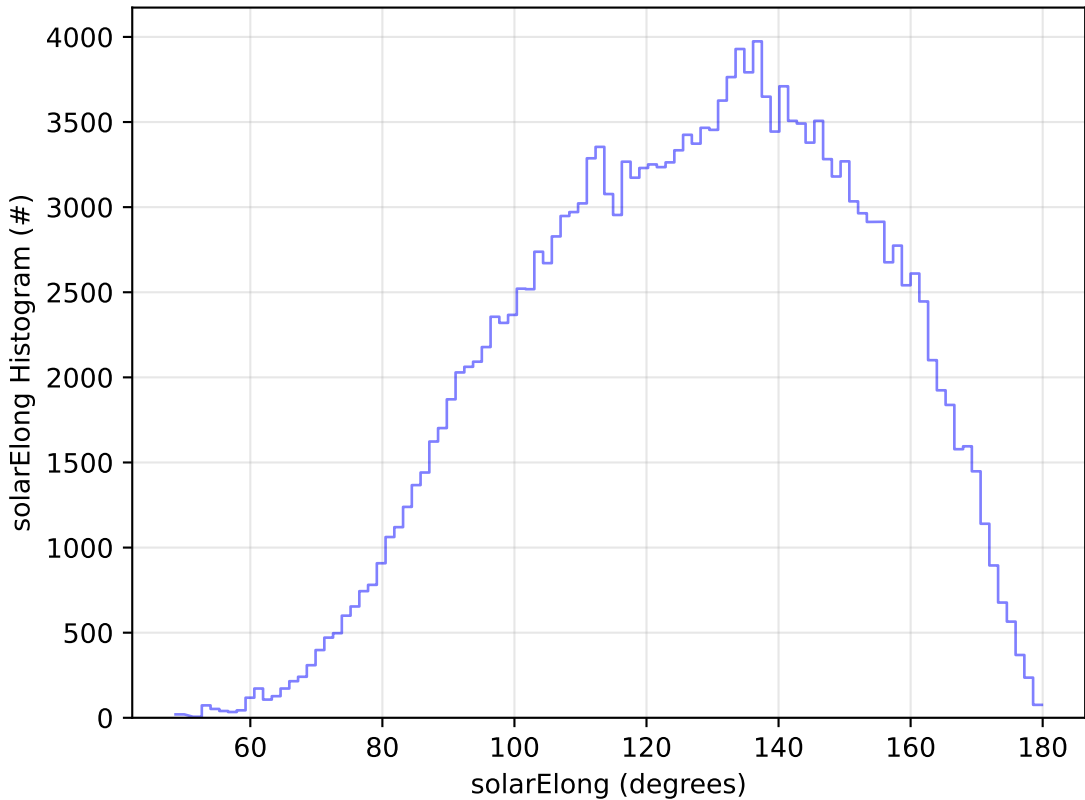
ddf_acor_sf10_lsf30_lsr10_v3.4_10yrs WFD g band: solarElong Histogram
