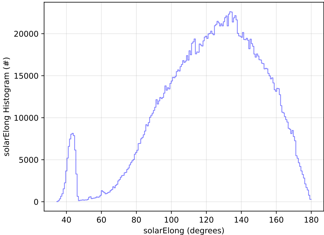
ddf_acor_sf10_lsf30_lsr10_v3.4_10yrs WFD all bands: solarElong Histogram
