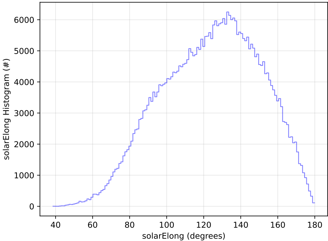
ddf_acor_sf10_lsf30_lsr10_v3.4_10yrs All sky y band: solarElong Histogram
