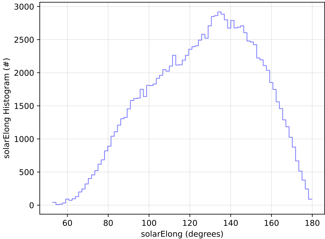
ddf_acor_sf10_lsf30_lsr10_v3.4_10yrs All sky u band: solarElong Histogram
