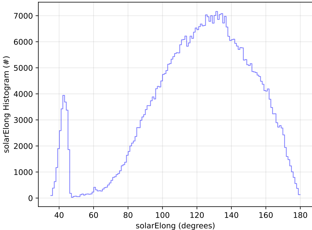
ddf_acor_sf10_lsf30_lsr10_v3.4_10yrs All sky i band: solarElong Histogram
