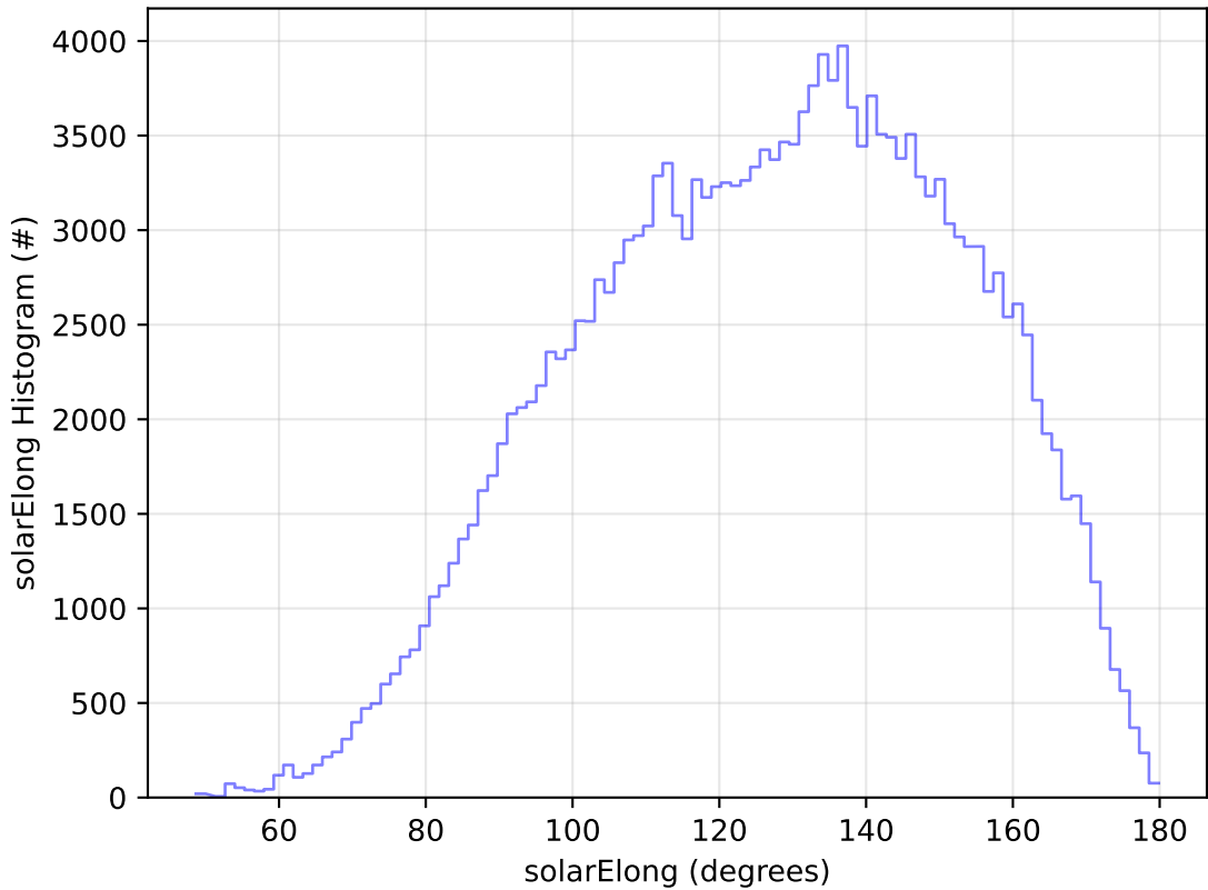
ddf_acor_sf10_lsf30_lsr10_v3.4_10yrs All sky g band: solarElong Histogram
