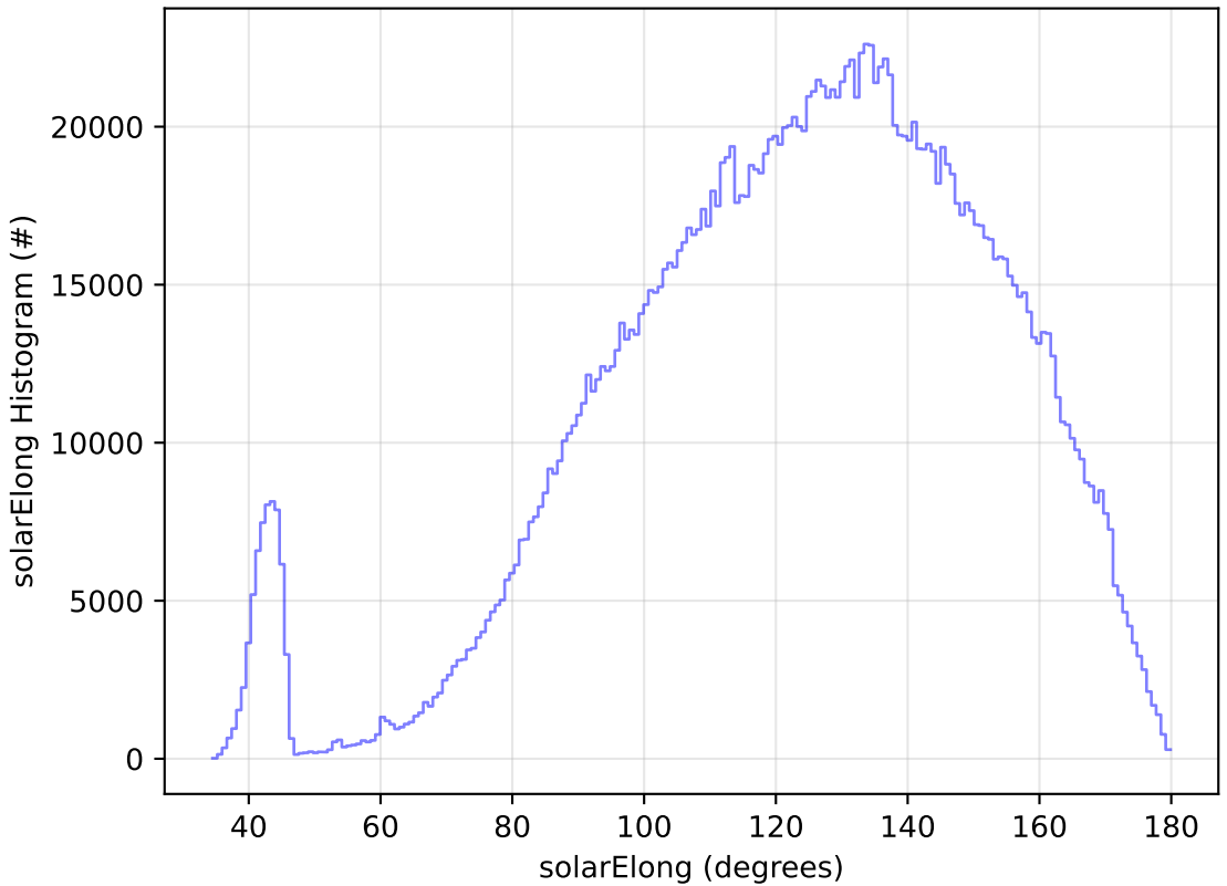
ddf_acor_sf10_lsf30_lsr10_v3.4_10yrs All sky all bands: solarElong Histogram
