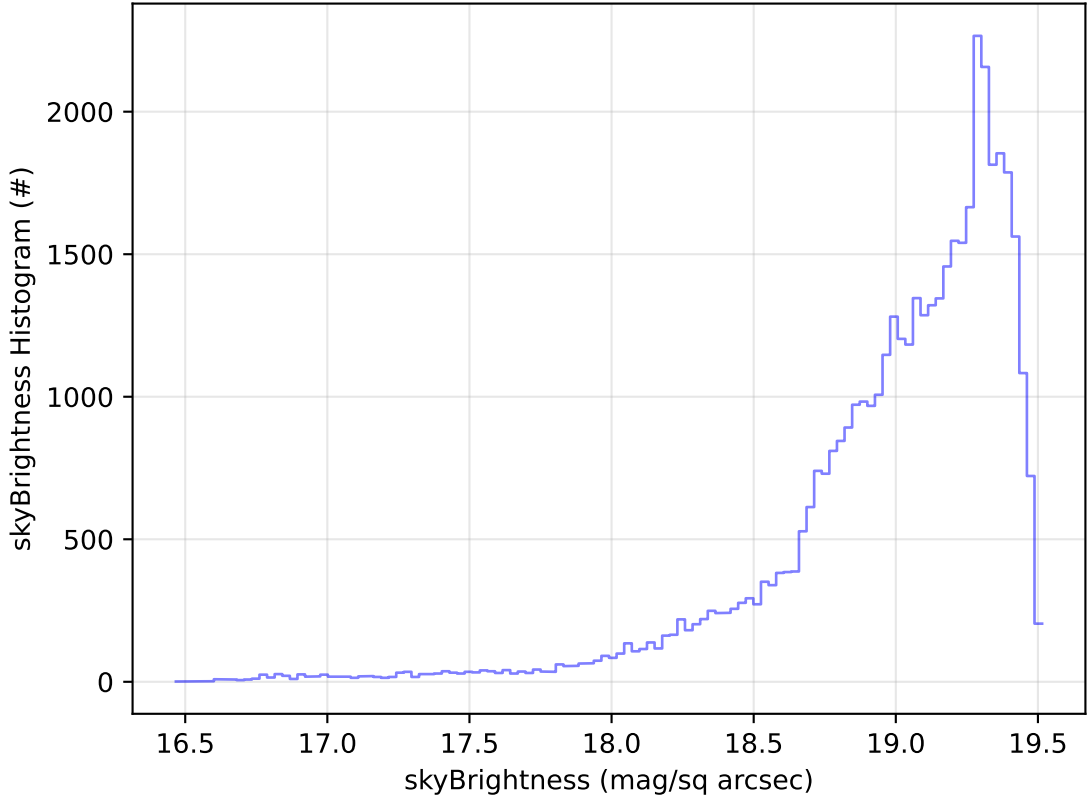
ddf_acor_sf10_lsf30_lsr10_v3.4_10yrs Yr 1 z band: skyBrightness Histogram
