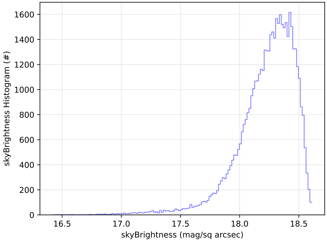
ddf_acor_sf10_lsf30_lsr10_v3.4_10yrs Yr 1 y band: skyBrightness Histogram
