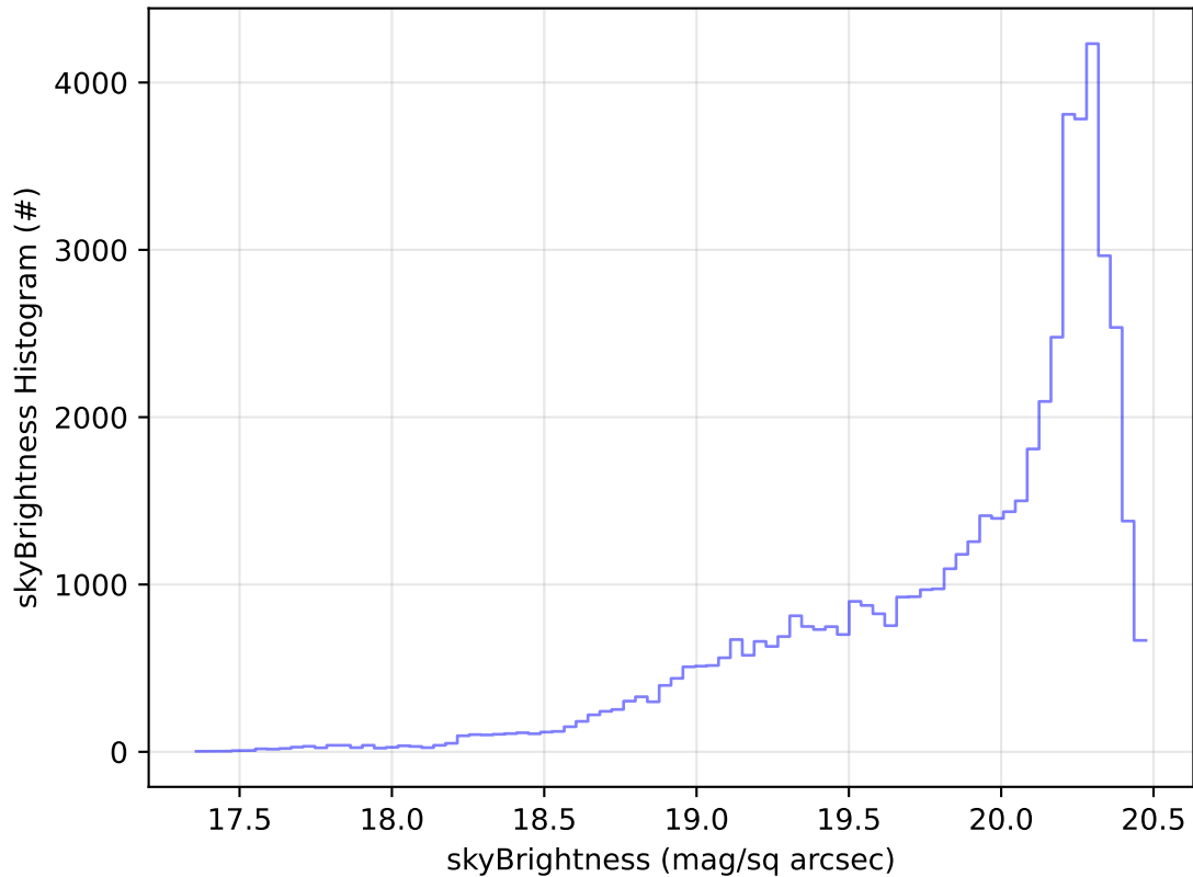
ddf_acor_sf10_lsf30_lsr10_v3.4_10yrs Yr 1 i band: skyBrightness Histogram
