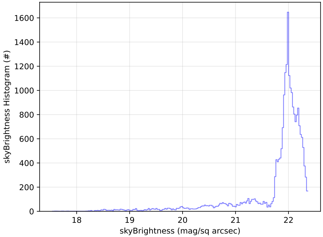
ddf_acor_sf10_lsf30_lsr10_v3.4_10yrs Yr 1 g band: skyBrightness Histogram
