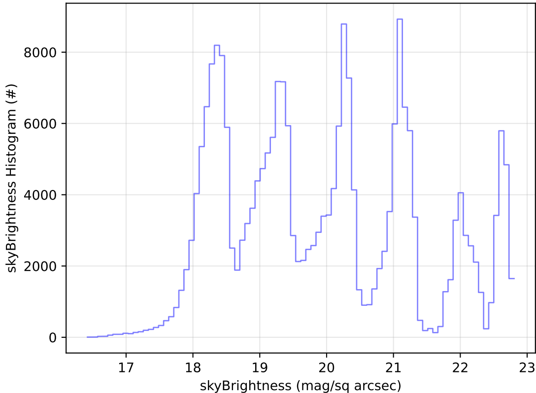
ddf_acor_sf10_lsf30_lsr10_v3.4_10yrs Yr 1 all bands: skyBrightness Histogram
