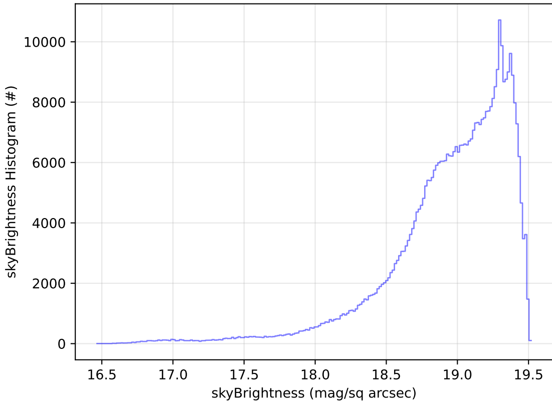
ddf_acor_sf10_lsf30_lsr10_v3.4_10yrs WFD z band: skyBrightness Histogram
