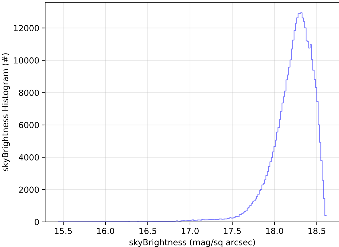
ddf_acor_sf10_lsf30_lsr10_v3.4_10yrs WFD y band: skyBrightness Histogram
