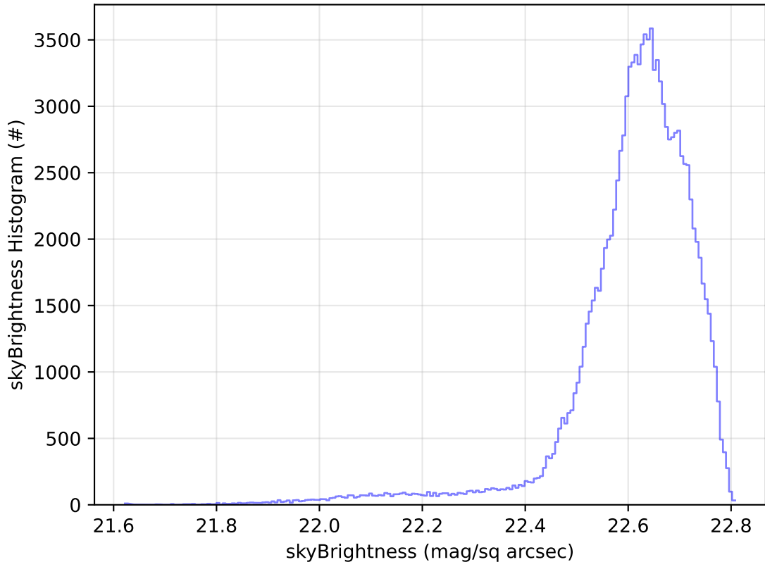
ddf_acor_sf10_lsf30_lsr10_v3.4_10yrs WFD u band: skyBrightness Histogram
