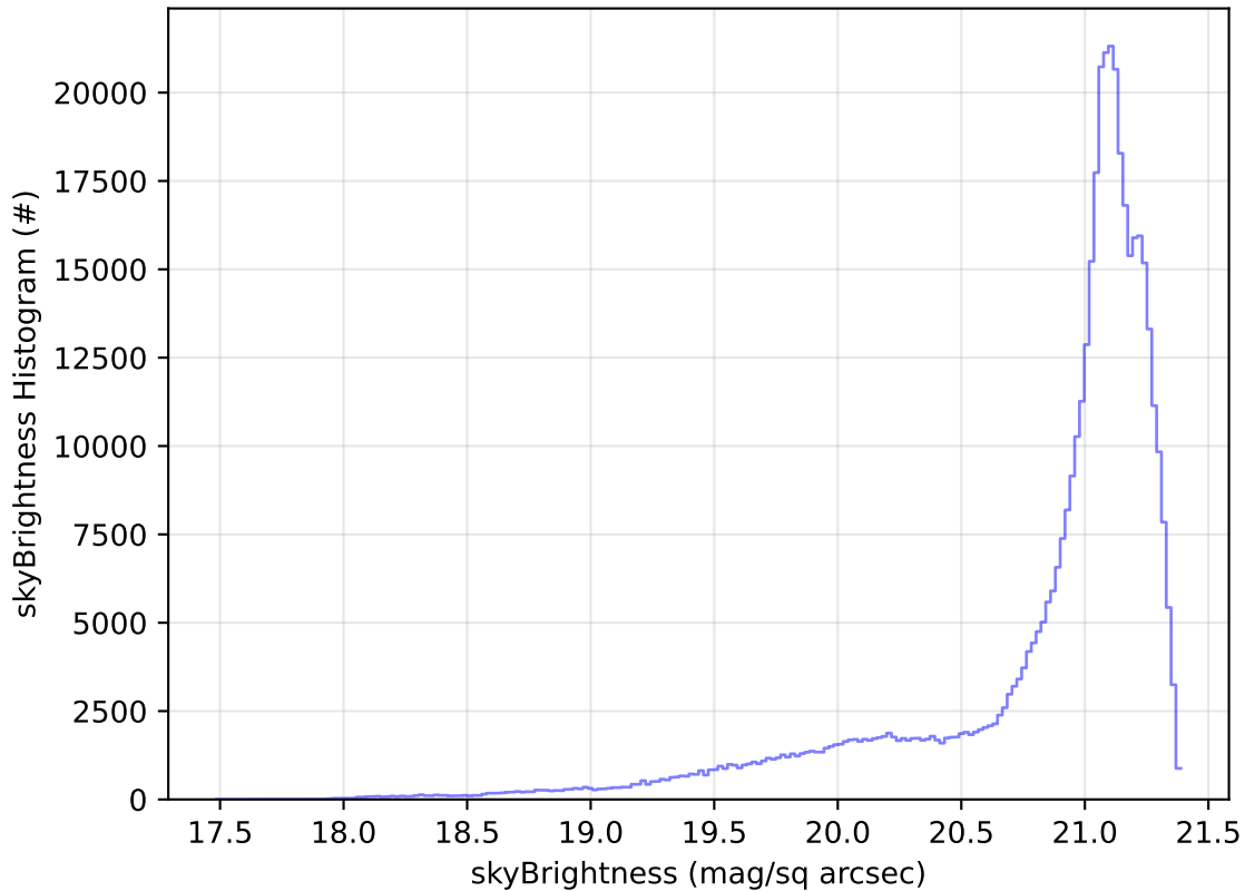
ddf_acor_sf10_lsf30_lsr10_v3.4_10yrs WFD r band: skyBrightness Histogram
