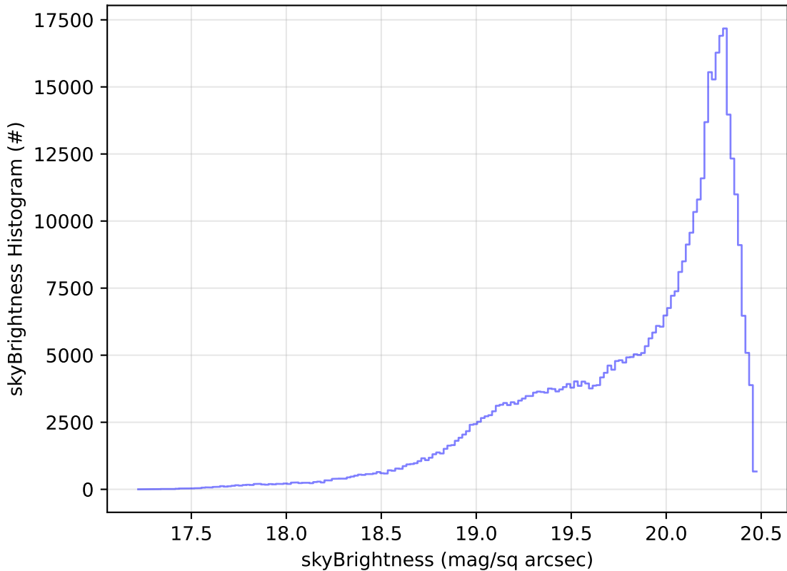
ddf_acor_sf10_lsf30_lsr10_v3.4_10yrs WFD i band: skyBrightness Histogram
