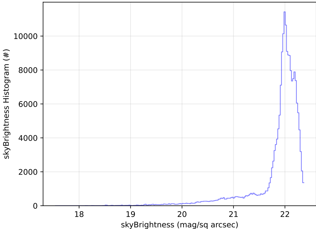
ddf_acor_sf10_lsf30_lsr10_v3.4_10yrs WFD g band: skyBrightness Histogram
