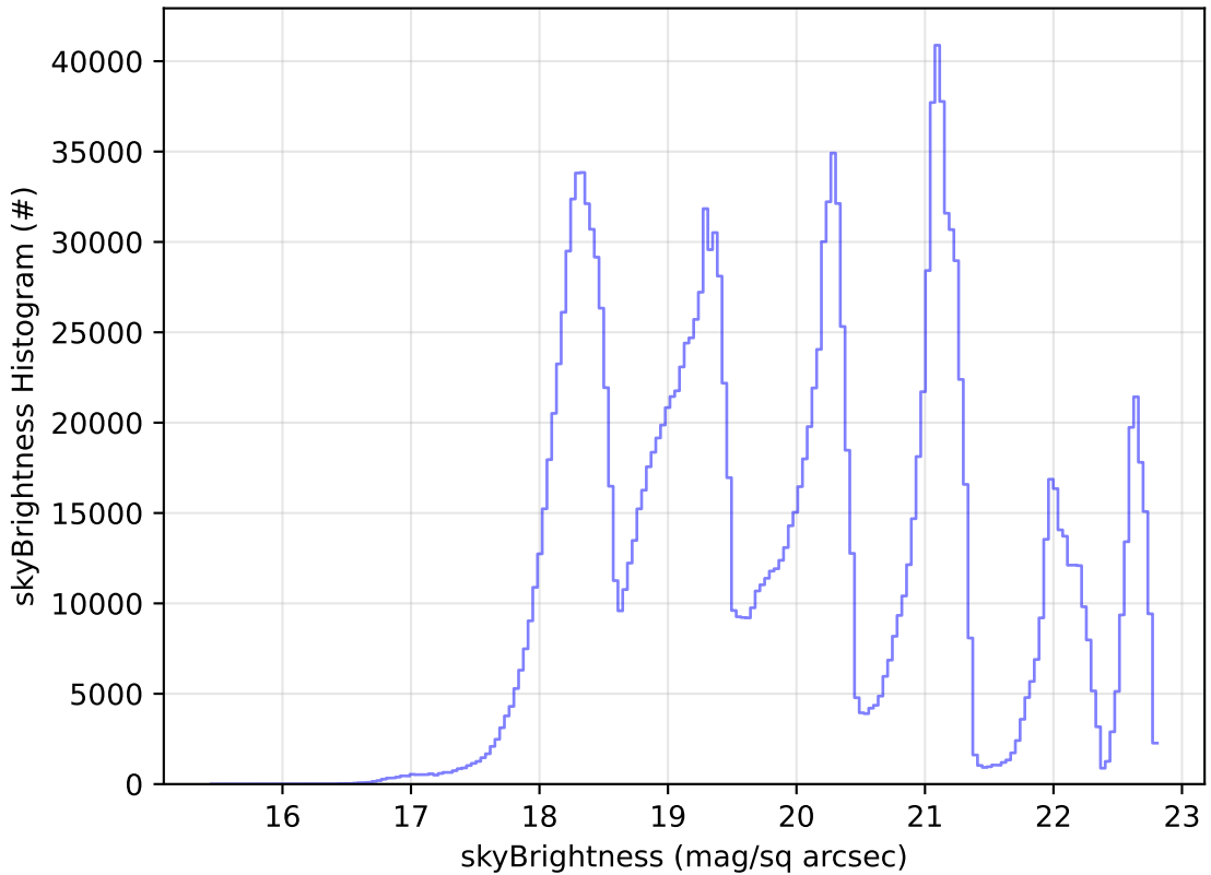
ddf_acor_sf10_lsf30_lsr10_v3.4_10yrs WFD all bands: skyBrightness Histogram
