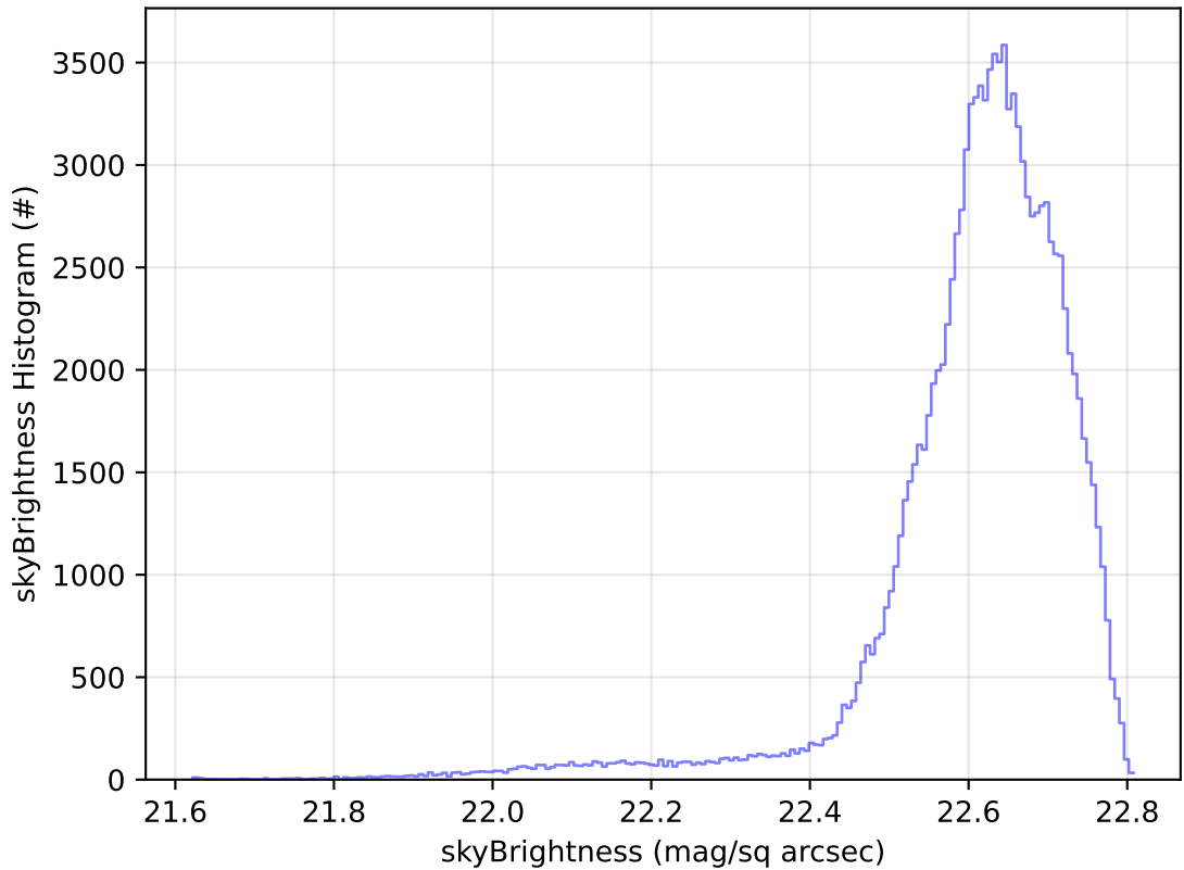
ddf_acor_sf10_lsf30_lsr10_v3.4_10yrs All sky u band: skyBrightness Histogram
