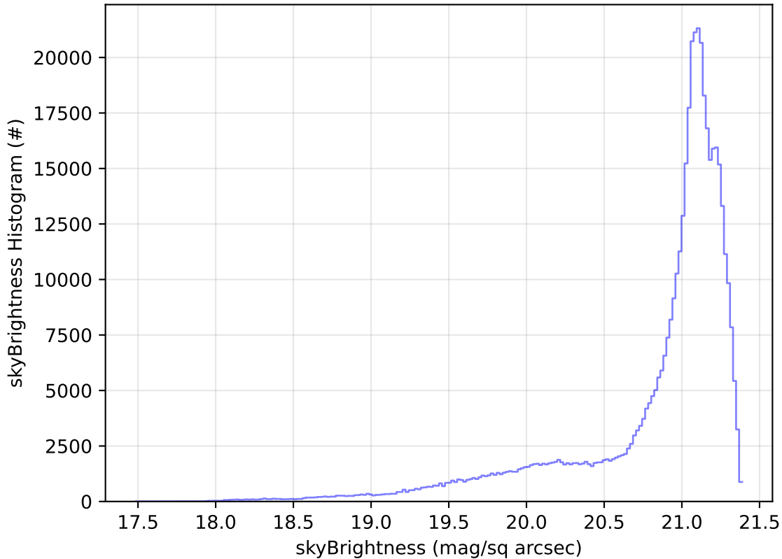
ddf_acor_sf10_lsf30_lsr10_v3.4_10yrs All sky r band: skyBrightness Histogram
