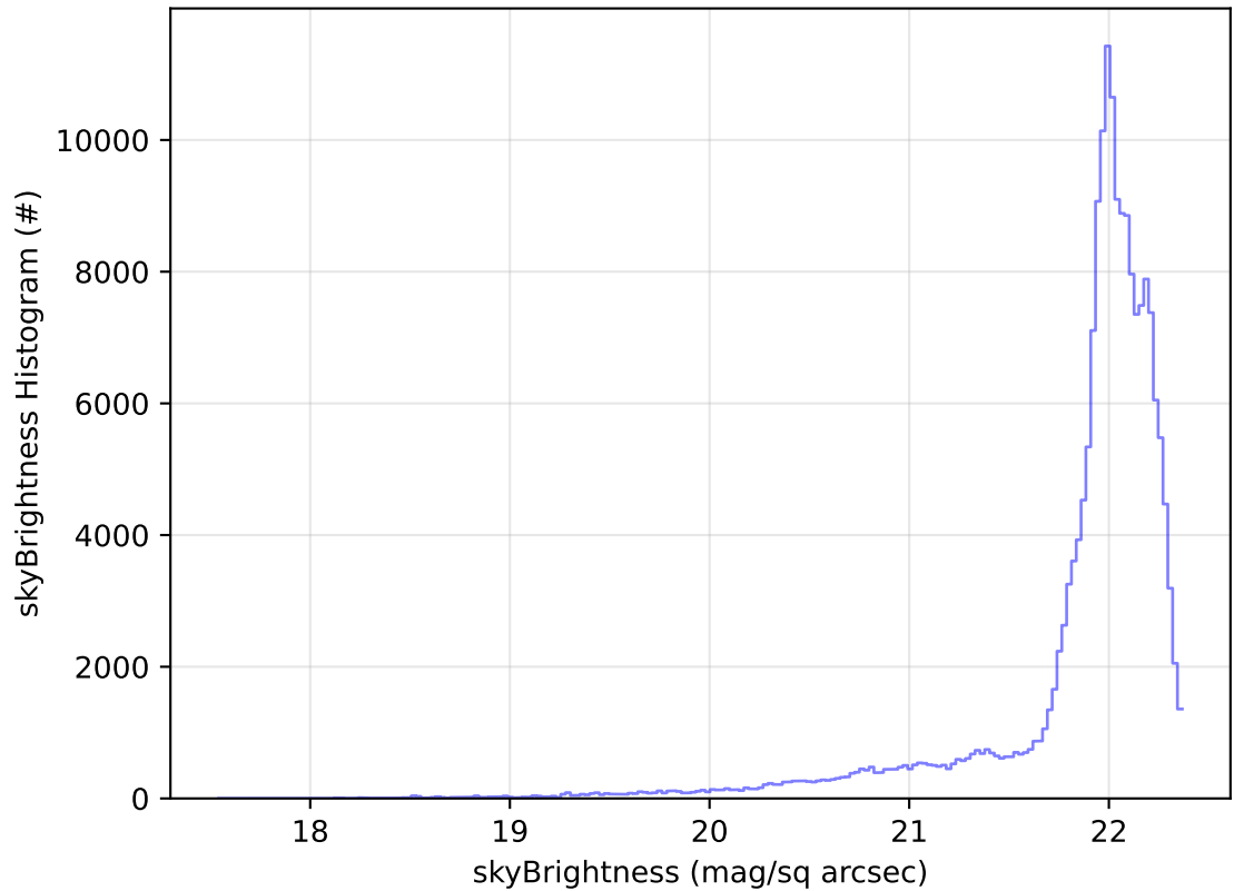
ddf_acor_sf10_lsf30_lsr10_v3.4_10yrs All sky g band: skyBrightness Histogram
