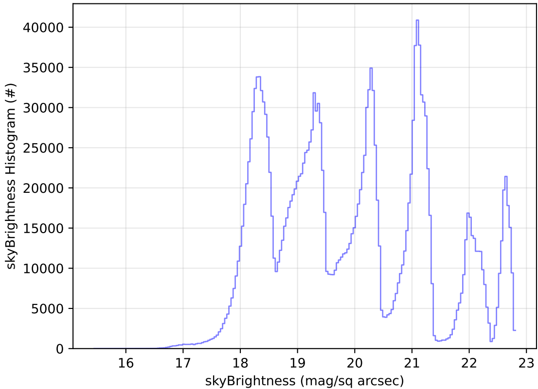
ddf_acor_sf10_lsf30_lsr10_v3.4_10yrs All sky all bands: skyBrightness Histogram
