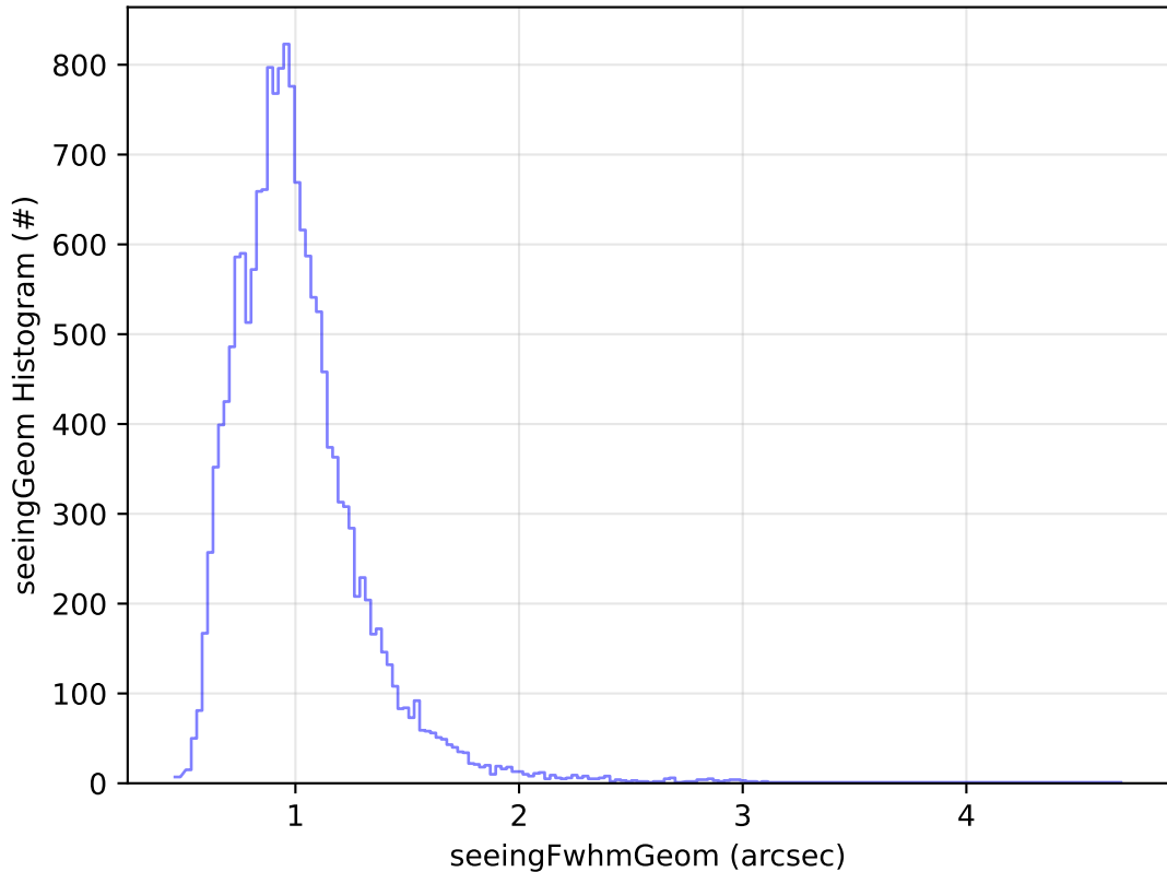
ddf_acor_sf10_lsf30_lsr10_v3.4_10yrs Yr 1 u band: seeingGeom Histogram
