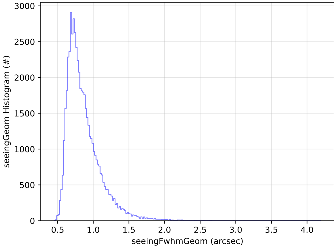
ddf_acor_sf10_lsf30_lsr10_v3.4_10yrs Yr 1 i band: seeingGeom Histogram
