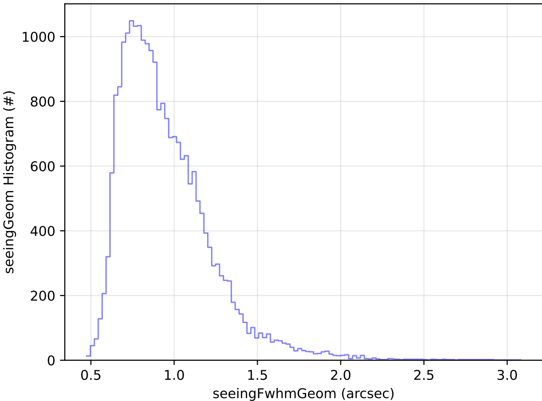
ddf_acor_sf10_lsf30_lsr10_v3.4_10yrs Yr 1 g band: seeingGeom Histogram
