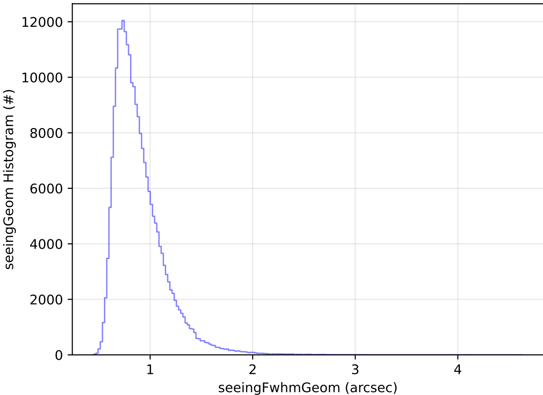
ddf_acor_sf10_lsf30_lsr10_v3.4_10yrs Yr 1 all bands: seeingGeom Histogram
