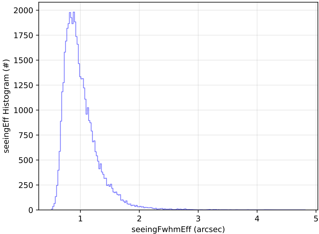
ddf_acor_sf10_lsf30_lsr10_v3.4_10yrs Yr 1 z band: seeingEff Histogram
