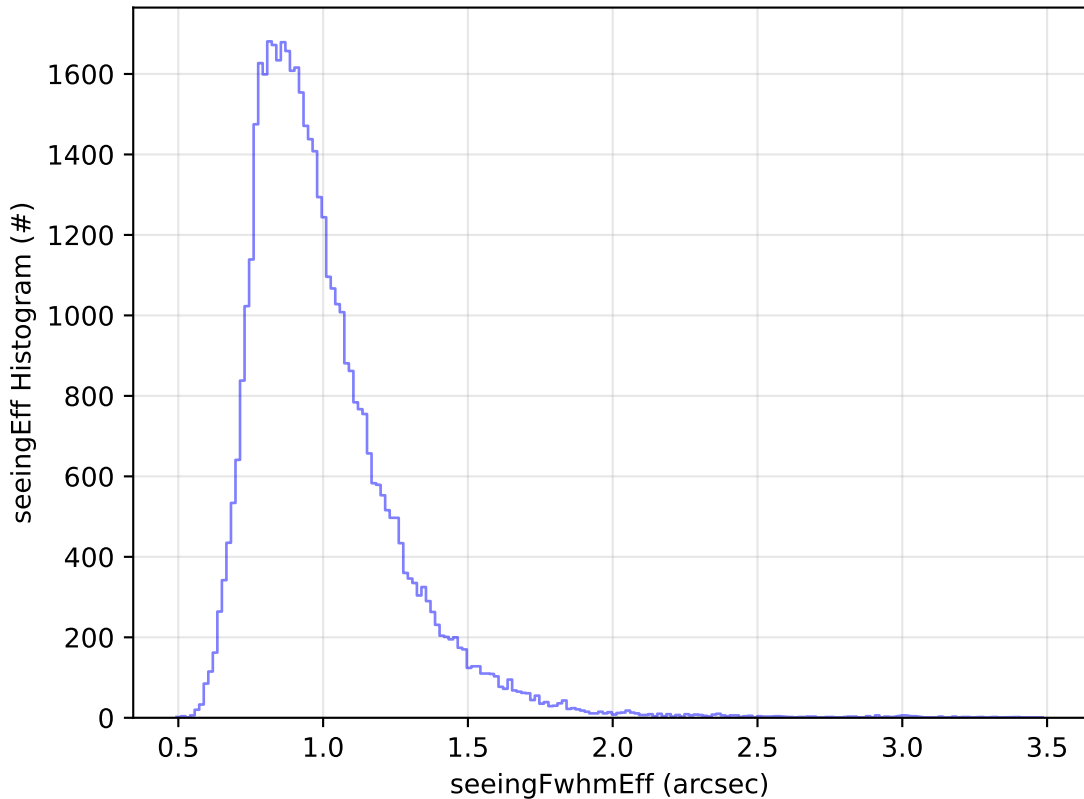
ddf_acor_sf10_lsf30_lsr10_v3.4_10yrs Yr 1 y band: seeingEff Histogram
