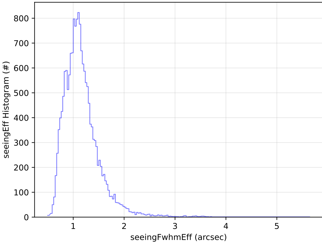
ddf_acor_sf10_lsf30_lsr10_v3.4_10yrs Yr 1 u band: seeingEff Histogram
