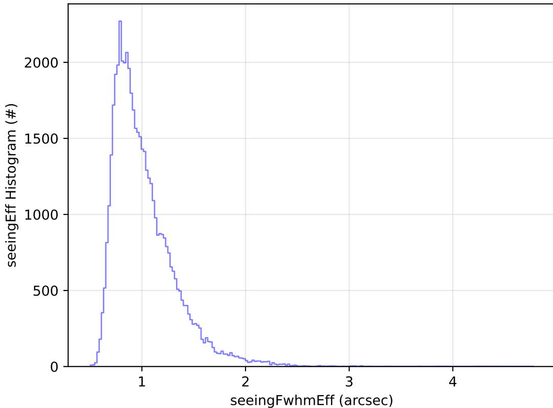
ddf_acor_sf10_lsf30_lsr10_v3.4_10yrs Yr 1 r band: seeingEff Histogram
