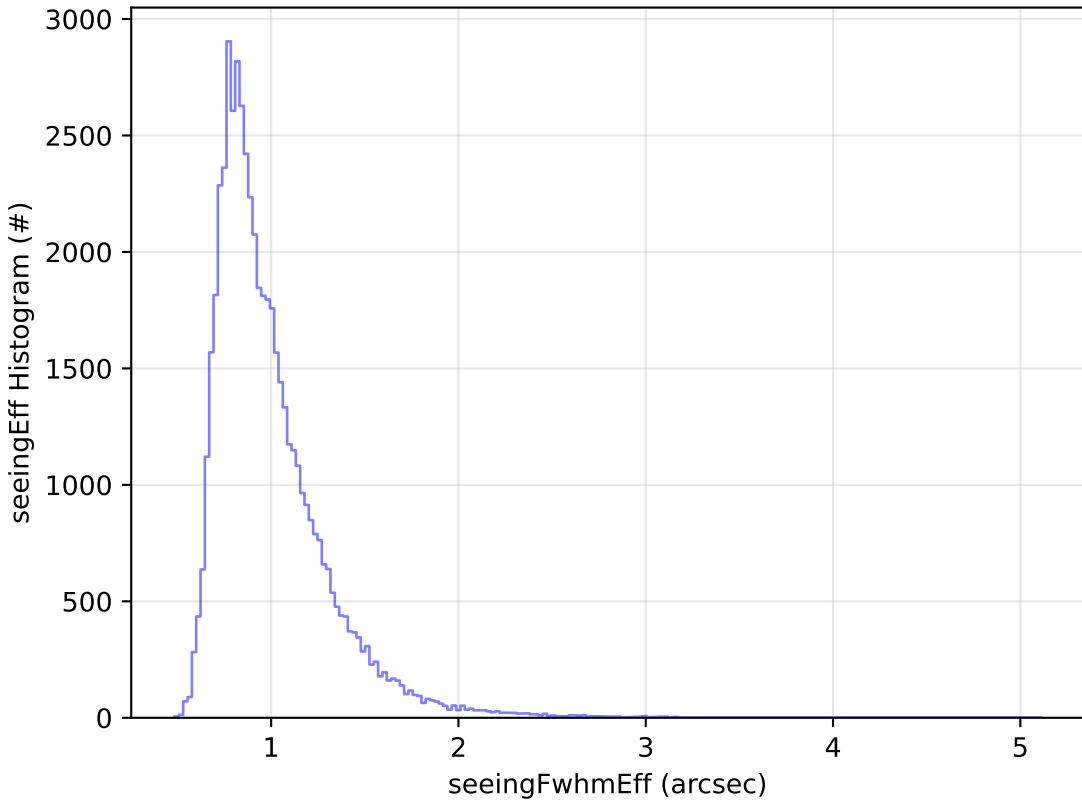
ddf_acor_sf10_lsf30_lsr10_v3.4_10yrs Yr 1 i band: seeingEff Histogram
