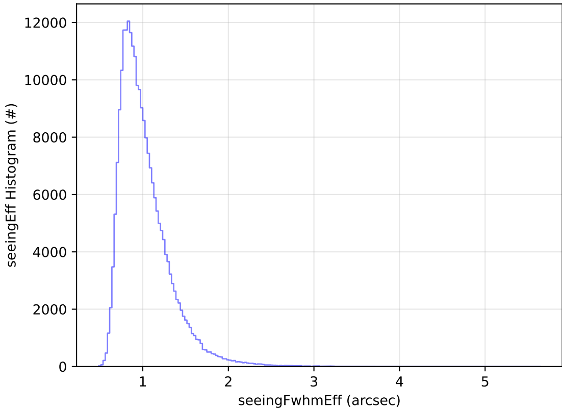
ddf_acor_sf10_Isf30_Isr10_v3.4_10yrs Yr 1 all bands: seeingEff Histogram
