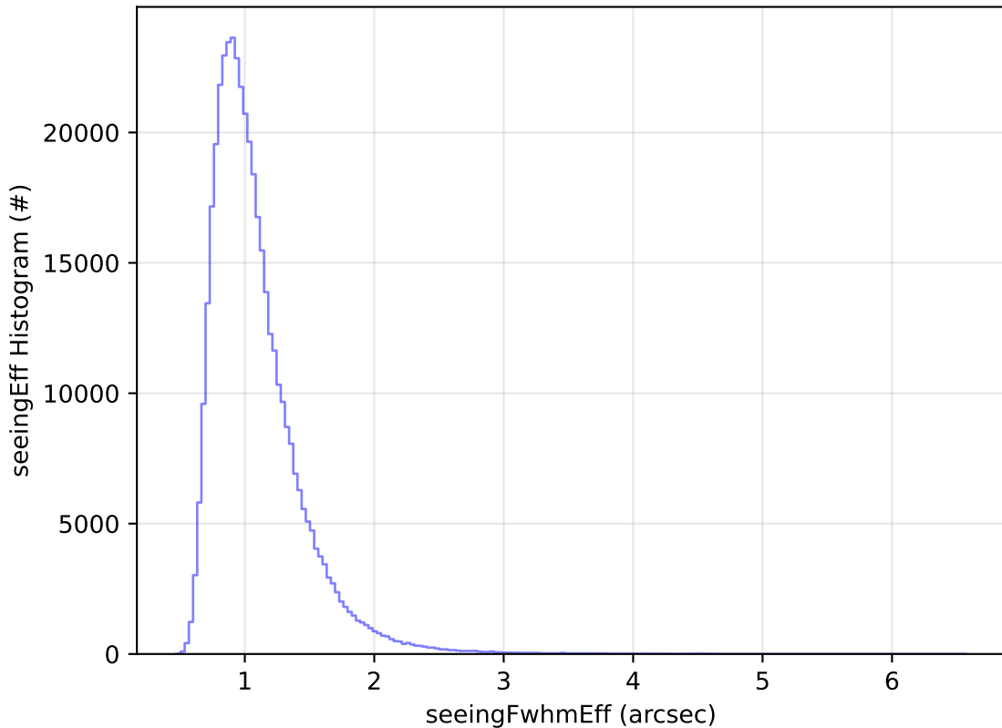
ddf_acor_sf10_lsf30_lsr10_v3.4_10yrs WFD z band: seeingEff Histogram
