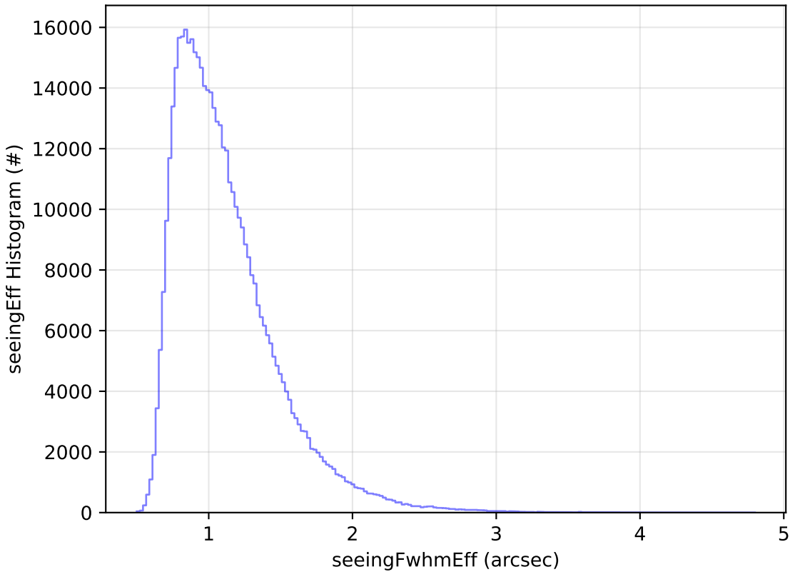
ddf_acor_sf10_lsf30_lsr10_v3.4_10yrs WFD r band: seeingEff Histogram
