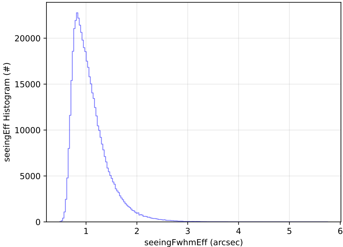
ddf_acor_sf10_lsf30_lsr10_v3.4_10yrs WFD i band: seeingEff Histogram
