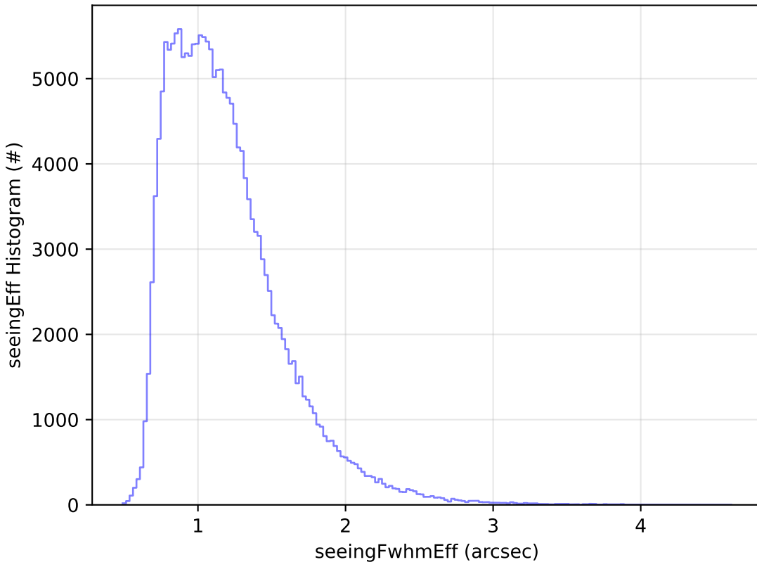
ddf_acor_sf10_lsf30_lsr10_v3.4_10yrs WFD g band: seeingEff Histogram
