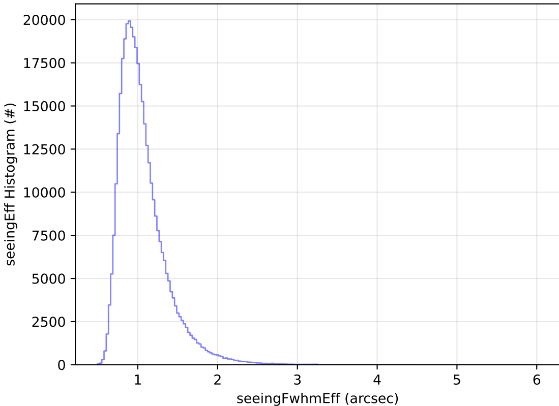
ddf_acor_sf10_lsf30_lsr10_v3.4_10yrs All sky y band: seeingEff Histogram
