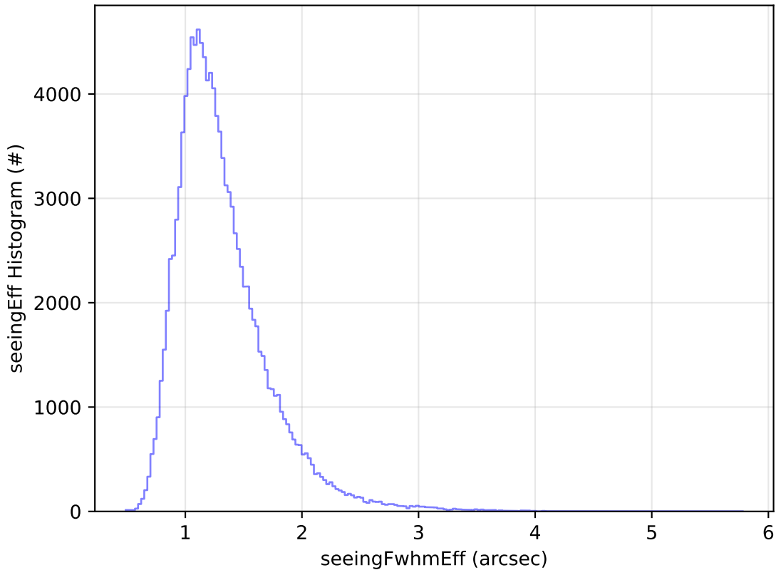
ddf_acor_sf10_ls30_lsr10_v3.4_10yrs All sky u band: seeingEff Histogram
