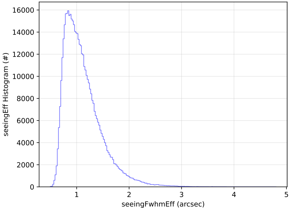
ddf_acor_sf10_lsf30_lsr10_v3.4_10yrs All sky r band: seeingEff Histogram
