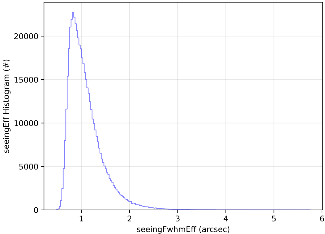
ddf_acor_sf10_lsf30_lsr10_v3.4_10yrs All sky i band: seeingEff Histogram
