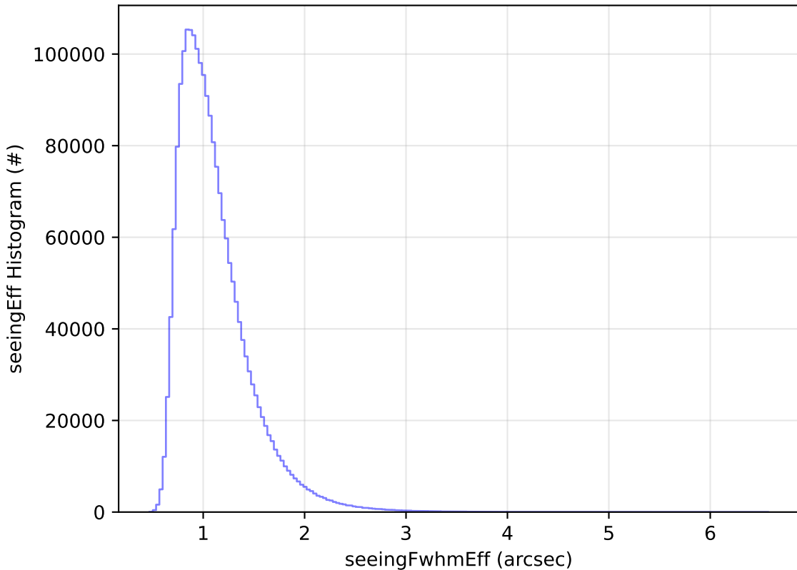
ddf_acor_sf10_lsf30_lsr10_v3.4_10yrs All sky all bands: seeingEff Histogram
