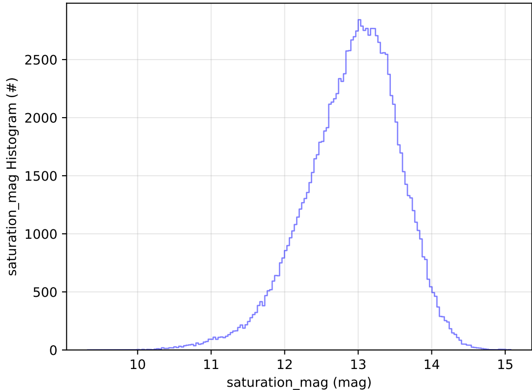
ddf_acor_sf10_lsf30_lsr10_v3.4_10yrs WFD u band: saturation_mag Histogram
