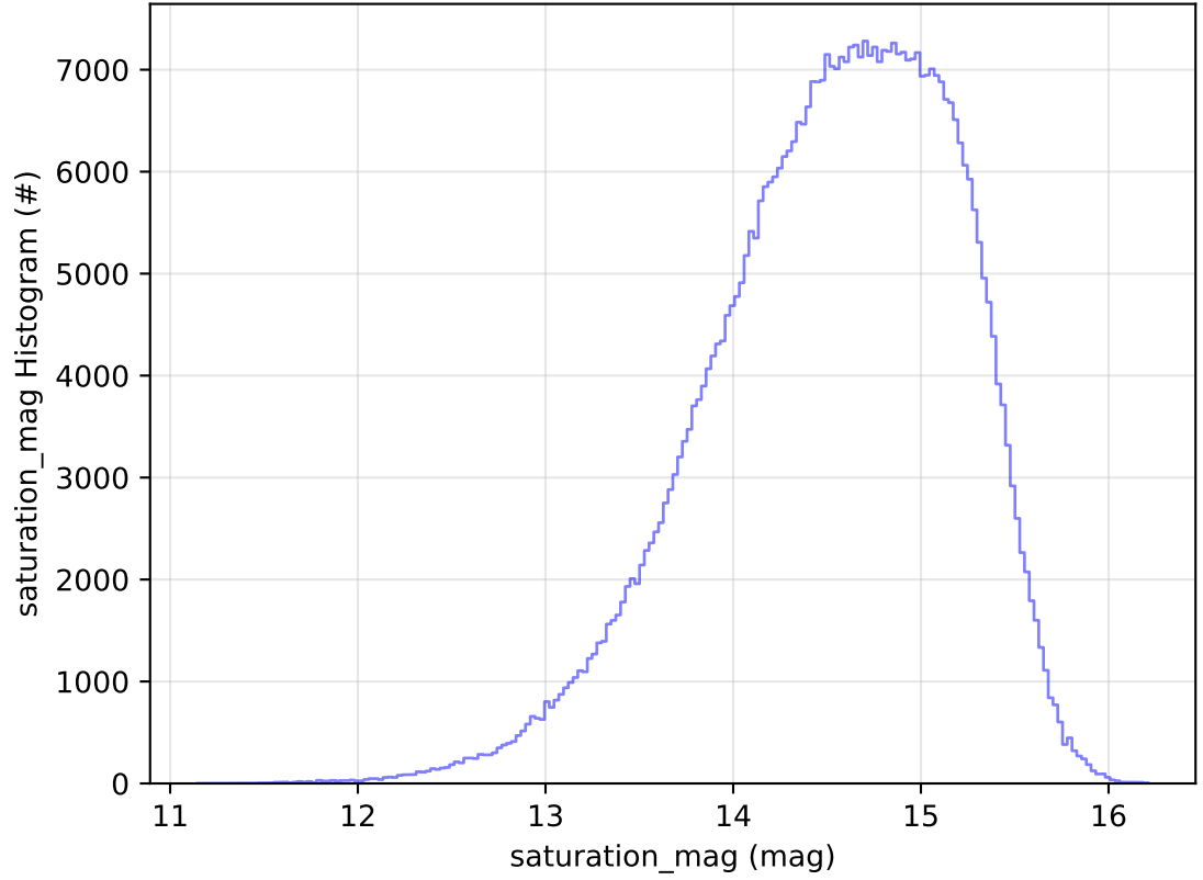
ddf_acor_sf10_lsf30_lsr10_v3.4_10yrs WFD r band: saturation_mag Histogram
