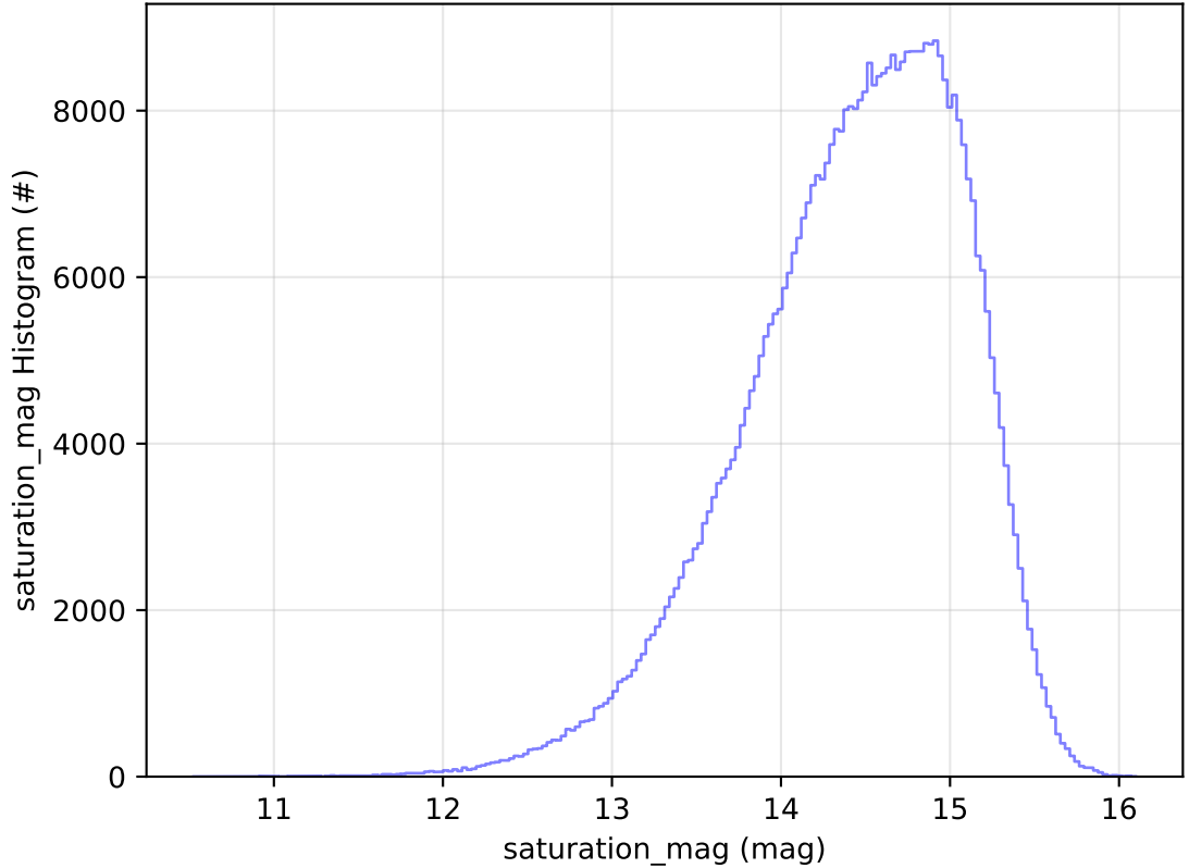
ddf_acor_sf10_lsf30_lsr10_v3.4_10yrs WFD i band: saturation_mag Histogram
