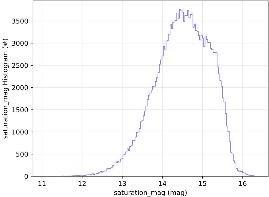
ddf_acor_sf10_lsf30_lsr10_v3.4_10yrs WFD g band: saturation_mag Histogram
